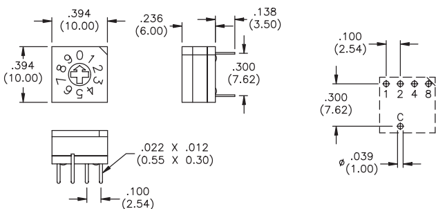
Mechanical outline
