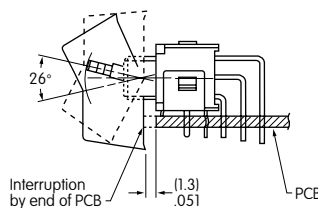
Side View of Rocker Vertical Mounting PC Single Pole and Double Pole
