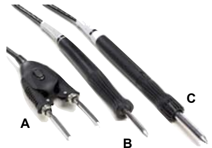
MFR-2200 Series Hand-pieces A. MFR-H4-TW Precision Tweezers B. MFR-H1-SC Soldering Cartridge C. MFR-H2-ST Soldering Tip
