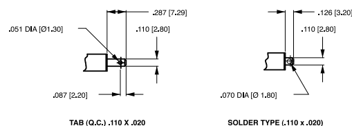
AUXILIARY SWITCH TERMINALS
