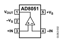
Figure 2. SOT-23-5 (RJ)
