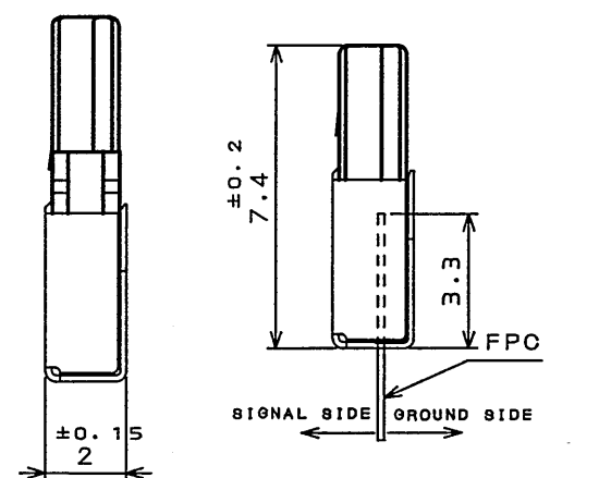
LOCKED CONDITION FPC嵌合状態図
