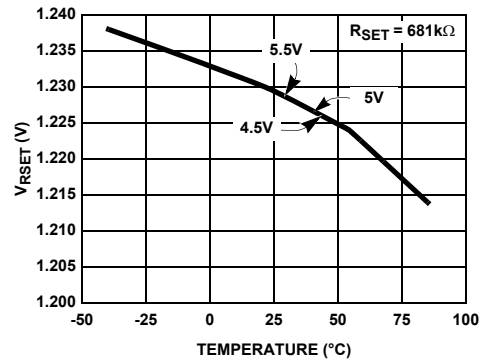
FIGURE 4. V_{RSET} vs TEMPERATURE
