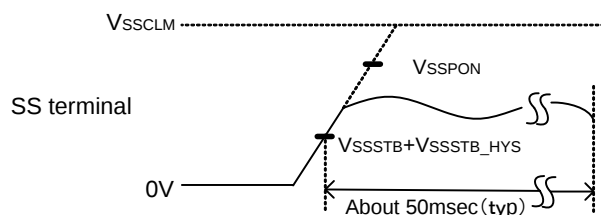
Figure.7 At soft start time-out
