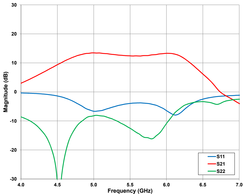
Figure 11. - Typical Small Signal Response V_{DD} = 20\text{ V} , I_{DQ} = 30\text{ mA}
