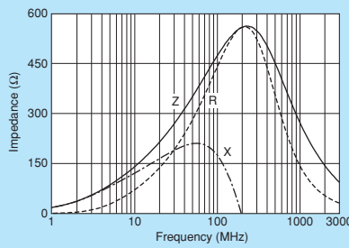
BLM18PG471SN1
