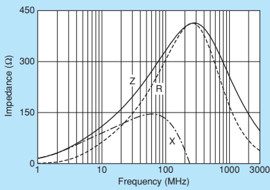
BLM18PG331SN1
