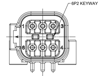
ATF13-6PX-BM1X VARIANTS
