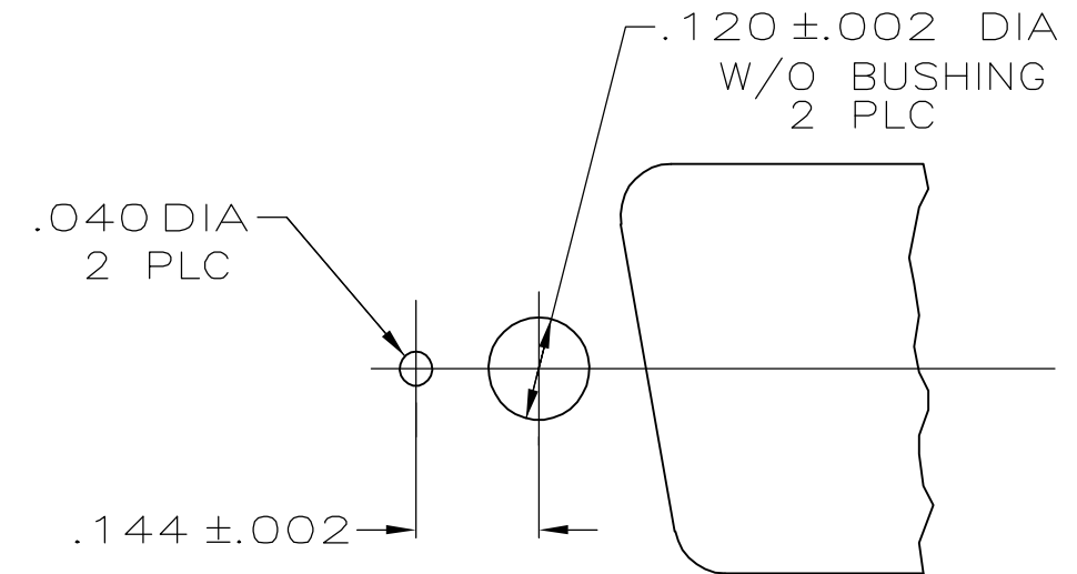
PANEL CUTOUT DETAIL NTS
