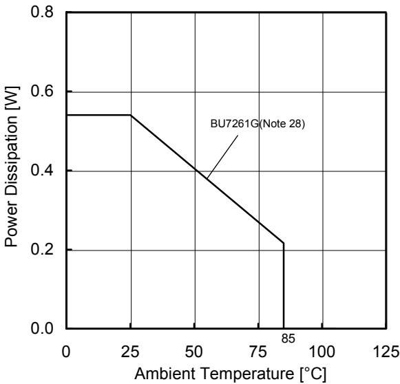
(c)BU7261G
