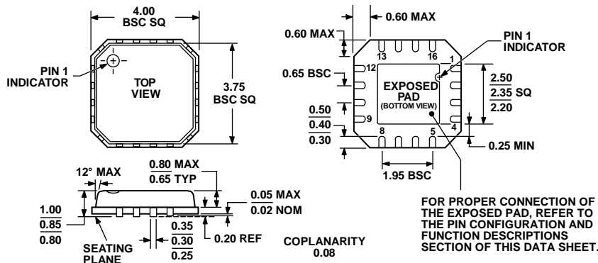
COMPLIANT TO JEDEC STANDARDS MO-220-VGGC Figure 64. 16-Lead Lead Frame Chip Scale Package [LFCSP_VQ] 4 mm x 4 mm Body, Very Thin Quad (CP-16-10) Dimensions shown in millimeters
