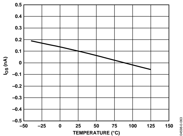
Figure 12. Input Offset Current vs. Temperature
