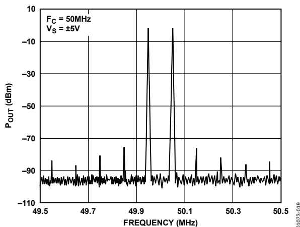
Figure 19. Intermodulation Distortion
