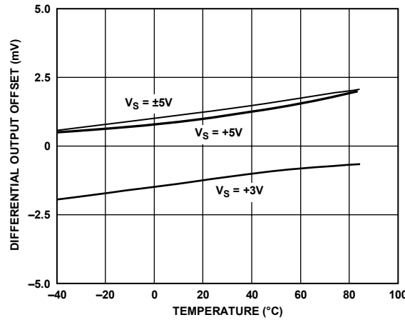
Figure 32. Output Referred Differential Offset Voltage vs. Temperature
