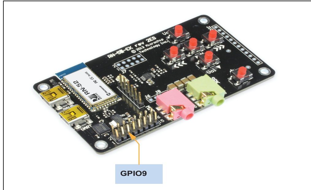
FIGURE 2-4: GPIO9 LOCATION
