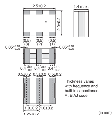
CSTCW_X11 20.01-48.00MHz
