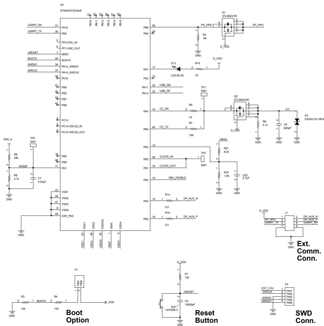
Figure 2. MCU section
