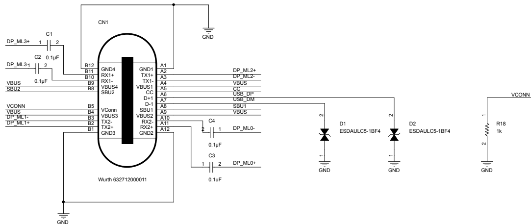
Figure 4. DisplayPort Receptacle
