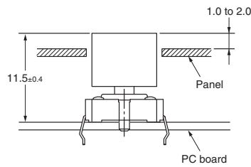
Reference Dimensions
