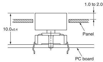
Reference Dimensions
