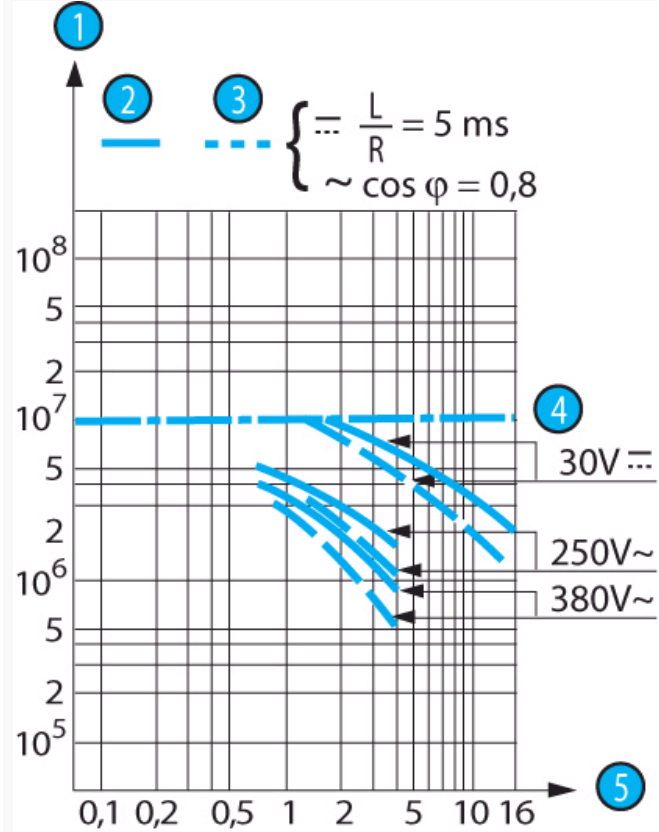
Operating curve for types 83 106 0 / 4 / 7
