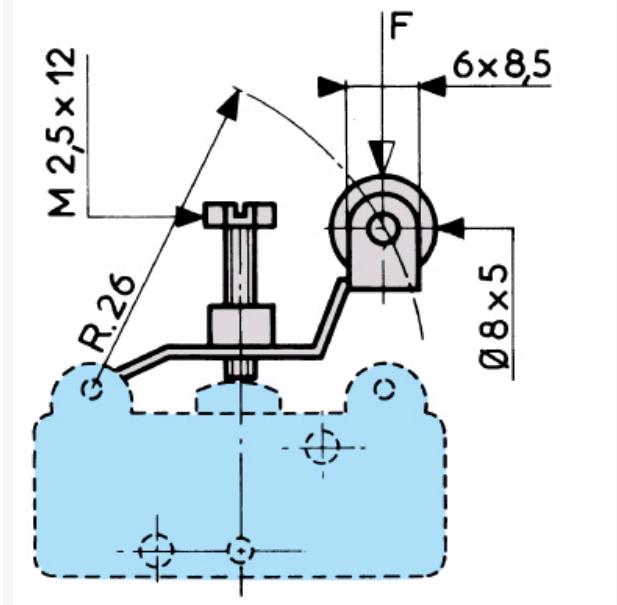
Lever cross-section 1 x 6.4 mm
