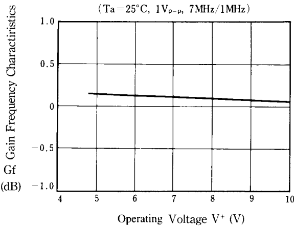
Gain Frequency Characteristics vs. Operating Voltage (Ta = 25°C, 1V P-P , 7MHz/1MHz)
