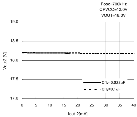
R1290K102A
