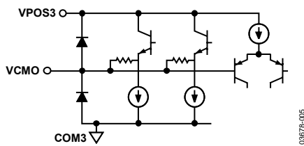
Figure 5. Circuit C
