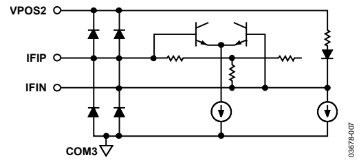
Figure 7. Circuit E
