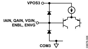
Figure 6. Circuit D
