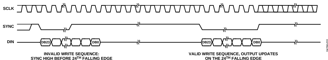
Figure 37. \overline{\text{SYNC}} Interrupt Facility
