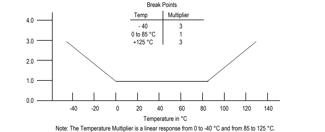
Figure 9. Temperature error multiplier (MPX5100D, MPX5100G, MPXV5100G)
