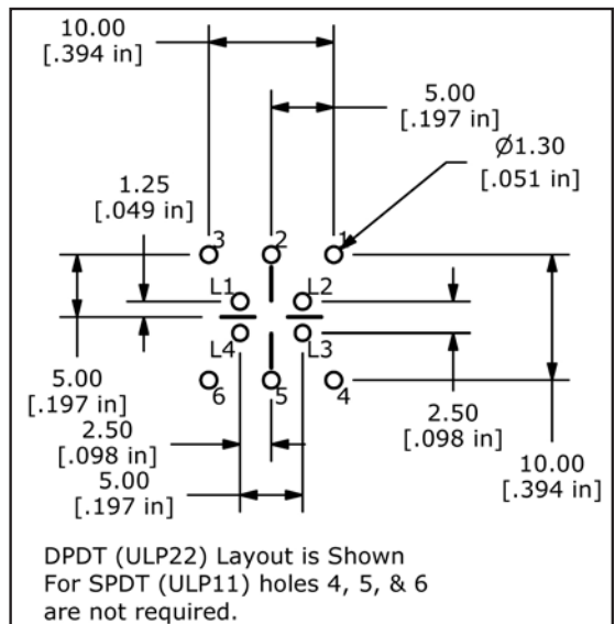
PCB LAYOUT - RGB LED
