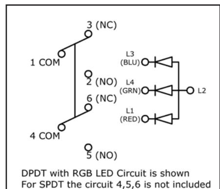
SCHEMATIC - RGB LED
