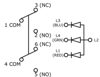
SCHEMATIC - RGB LED
