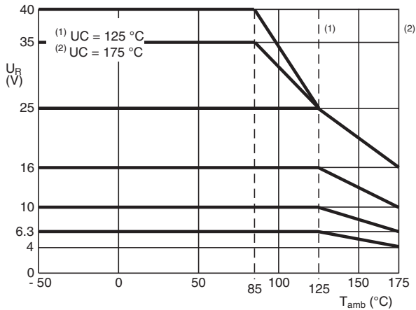
Fig. 3 - Maximum permissible voltage up to 175 ^{\circ}C
