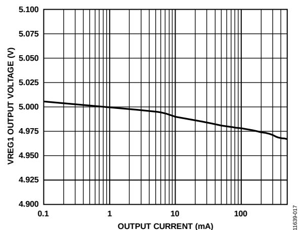
Figure 17. VREG1 Load Regulation
