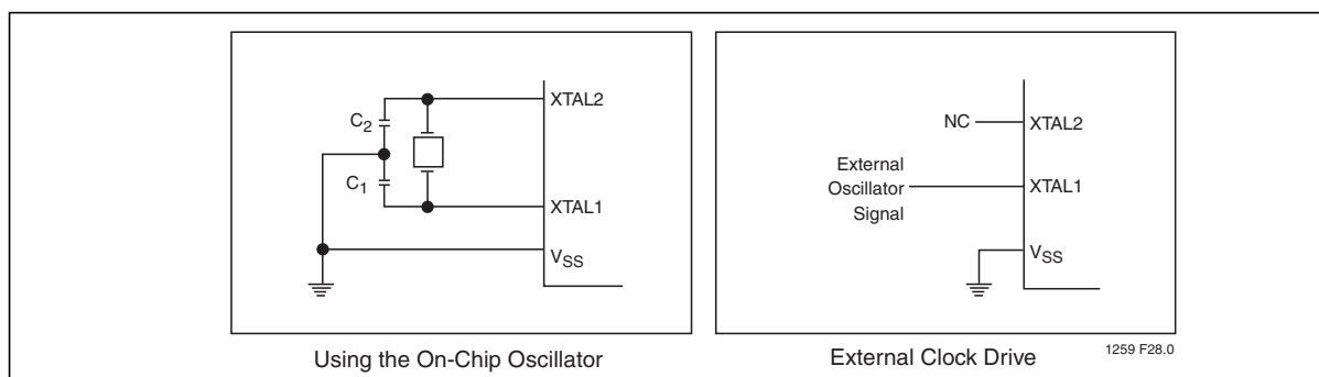
Figure 15: Oscillator Characteristics
