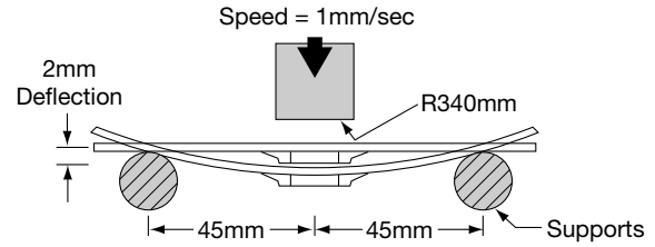
Figure 2. Bend Strength
