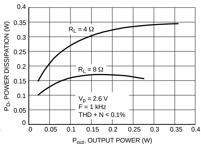
Figure 34. Power Dissipation versus Output Power
