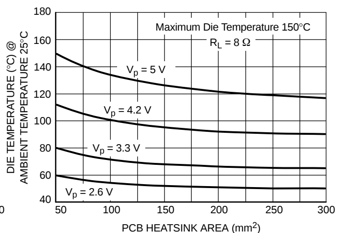
Figure 36. Maximum Die Temperature versus PCB Heatsink Area
