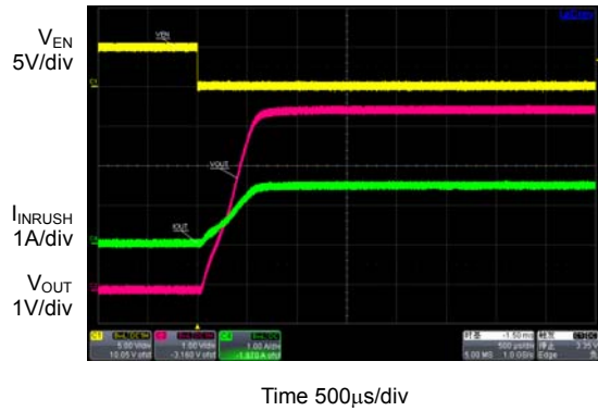
Figure 24. Output Turn On and Rise Time ( C_{IN}=1.0\mu F , C_{OUT}=1.0\mu F , R_L=3.3\Omega )
