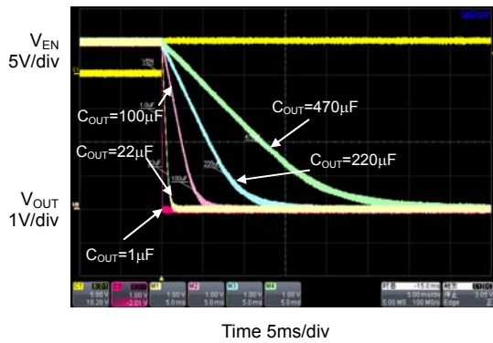
Figure 26. Output Turn Off and Fall Time ( V_{IN}=5V , C_{IN}=1.0\mu F , No Load)
