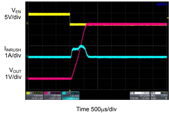
Figure 25. Output Turn On and Rise Time ( C_{IN}=1.0\mu F , C_{OUT}=100\mu F , No Load)
