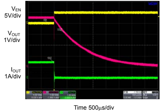
Figure 27. Output Turn Off and Fall Time ( V_{IN}=5V , C_{IN}=1.0\mu F , C_{OUT}=470\mu F , R_L=3.3\Omega )
