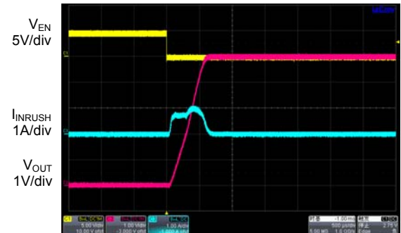
Time 500µs/div
