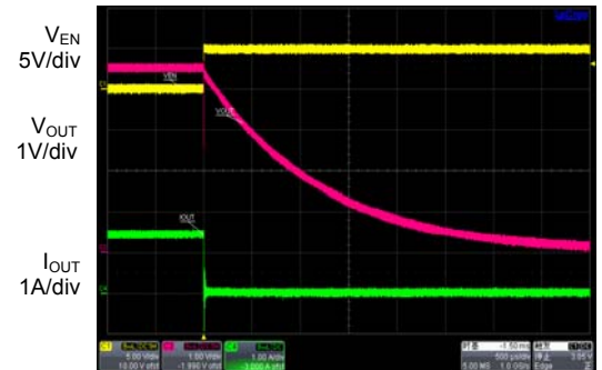
Time 500µs/div
