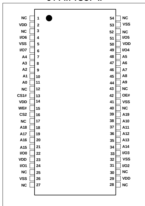
54-Pin TSOP-II
