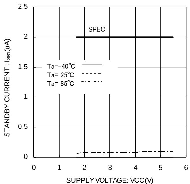
Figure 19. Standby current I_{SBI}(CS=0V, ORG=VCC \text{ or } OPEN)
