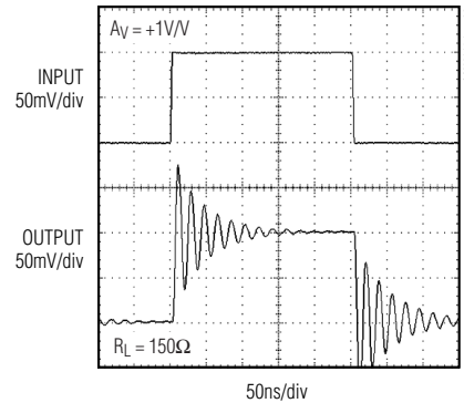
MAX4414/MAX4416/MAX4418 SMALL-SIGNAL PULSE RESPONSE ( C_{LOAD} = 15pF )
