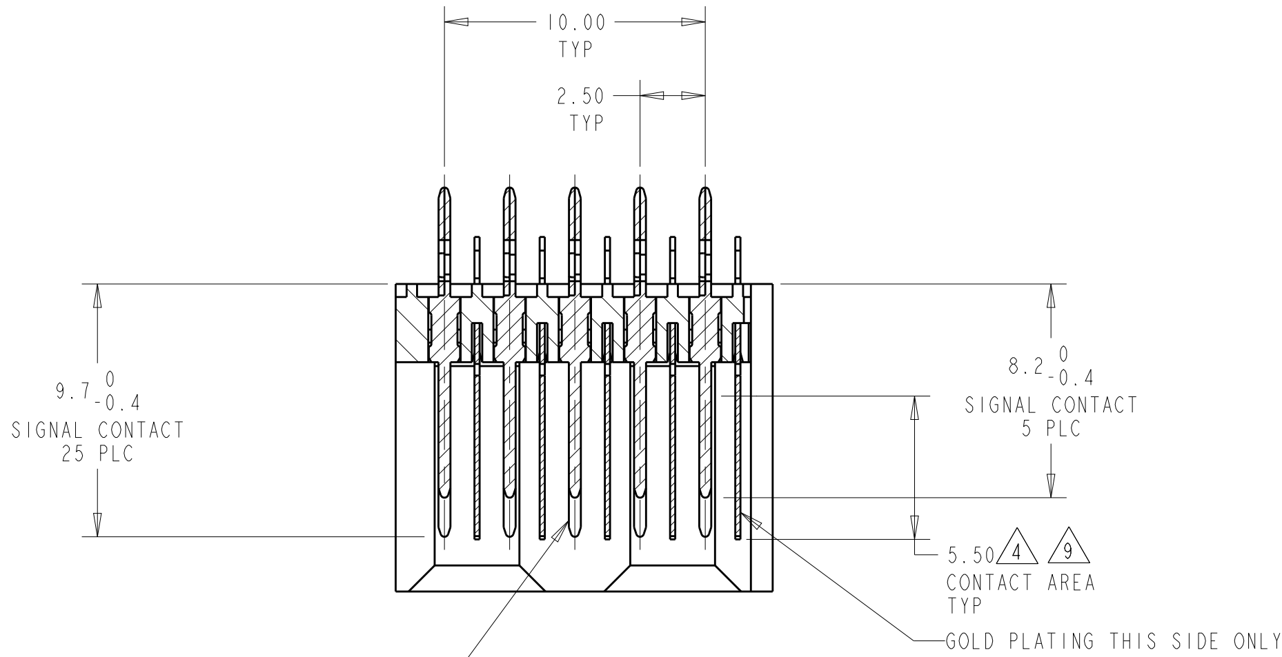
SECTION B-B
