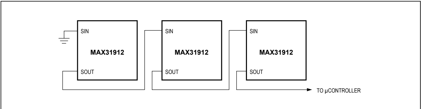
Figure 3. Daisy-Chain Operation
