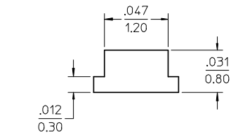
RECOMMENDED SMT 0603 LED DIMENSIONS SCALE 20:1 (SEE NOTE 1)
