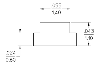
RECOMMENDED SMT 0805 LED DIMENSIONS SCALE 20:1 (SEE NOTE 1)
