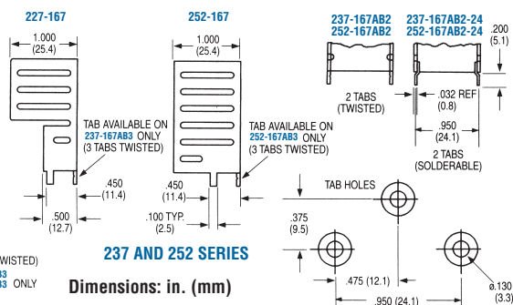
237 AND 252 SERIES Dimensions: in. (mm)
