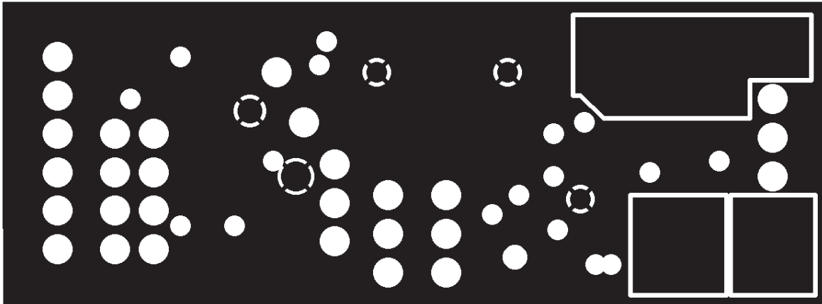
Figure 6. MAX9611PMB11 Peripheral Module PCB Layout—Inner Layer 2 (Power)
