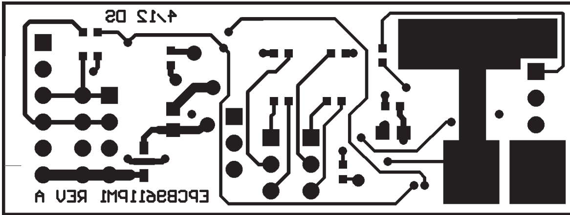
Figure 7. MAX9611PMB11 Peripheral Module PCB Layout—Solder Side
