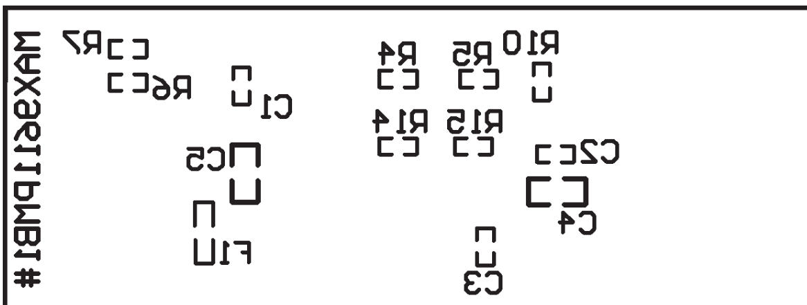
Figure 8. MAX9611PMB11 Peripheral Module Component Placement Guide—Solder Side
