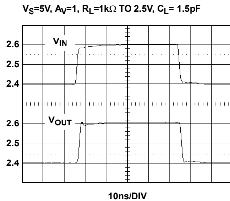
FIGURE 24. SMALL SIGNAL TRANSIENT REPNSE
