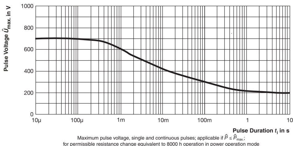
Pulse Voltage
