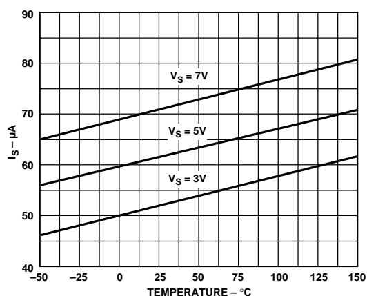
Figure 5. Supply Current vs. Temperature ( V_{OUT} = \text{HIGH} )
