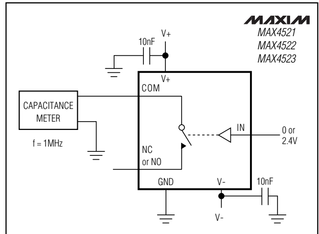
Figure 7. Channel On-Capacitance
