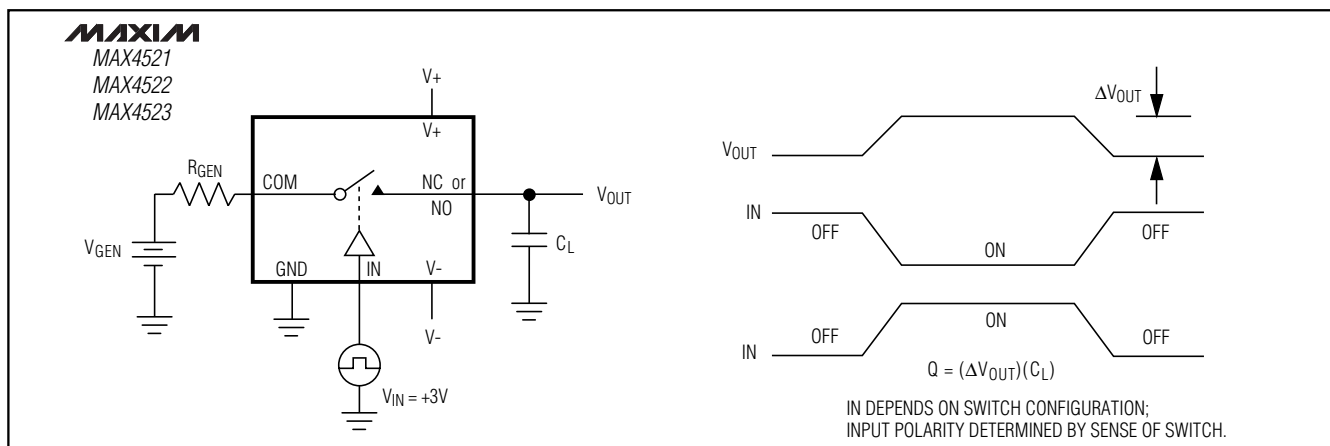
Figure 3. Charge Injection
