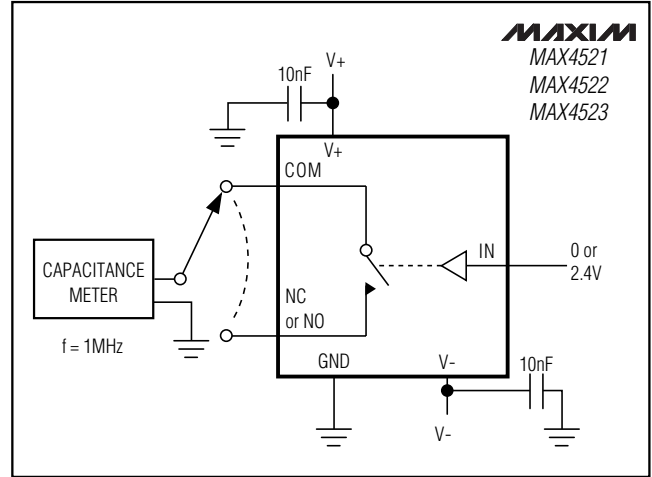
Figure 6. Channel Off-Capacitance
