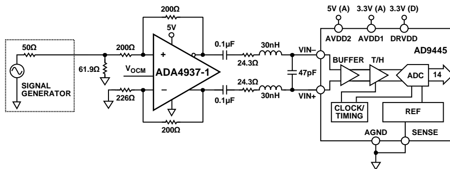
Figure 64. Driving an AD9445, 14-Bit, 105 MSPS ADC
