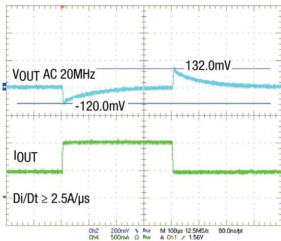
Figure 10. 12V_{IN} , 3.3V_{OUT} Transient Response, 0.5\text{A} to 1.0\text{A}
