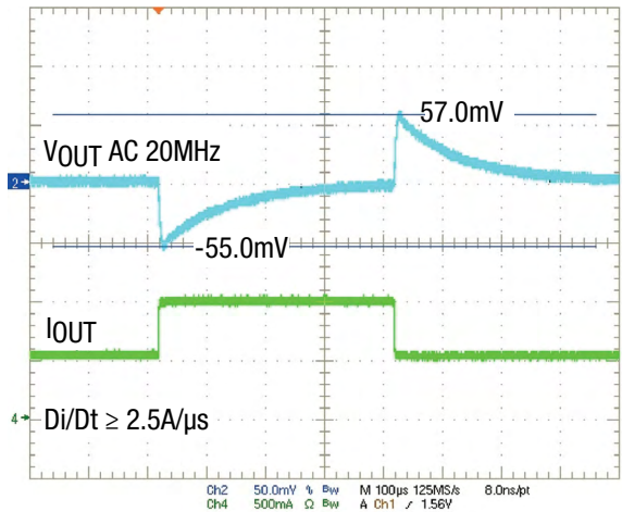
Figure 13. 5V_{IN} , 1.8V_{OUT} Transient Response, 0.5\text{A} to 1.0\text{A}
