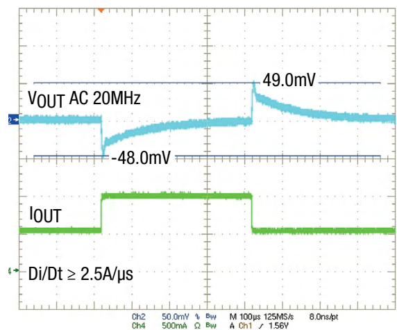
Figure 11. 12V_{IN} , 1.8V_{OUT} Transient Response, 0.5\text{A} to 1.0\text{A}
