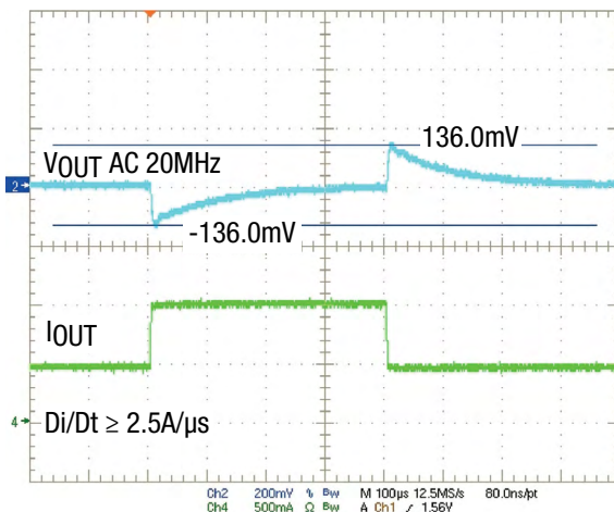
Figure 12. 5V_{IN} , 3.3V_{OUT} Transient Response, 0.5\text{A} to 1.0\text{A}
