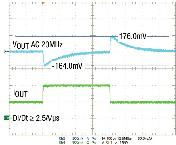
Figure 9. 12V_{IN} , 5.0V_{OUT} Transient Response, 0.5\text{A} to 1.0\text{A}
